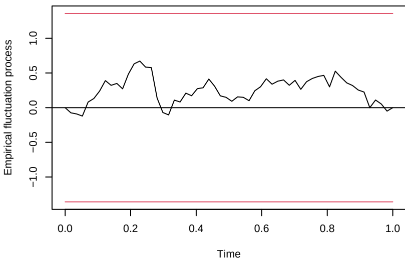
OLS-CUSUM of equation ipca
