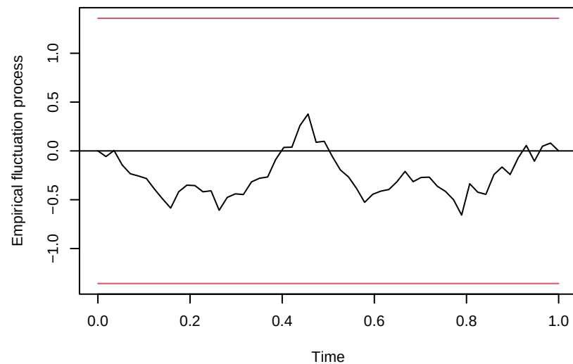
OLS-CUSUM of equation inad
