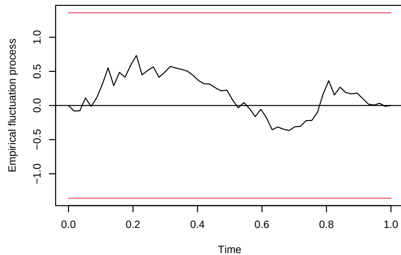
OLS-CUSUM of equation selic
