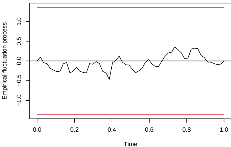
OLS-CUSUM of equation ibc
