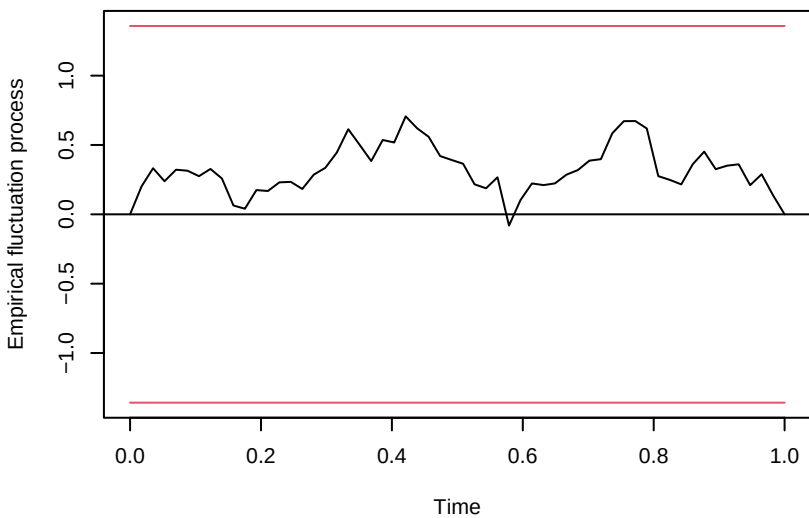
OLS-CUSUM of equation bets
